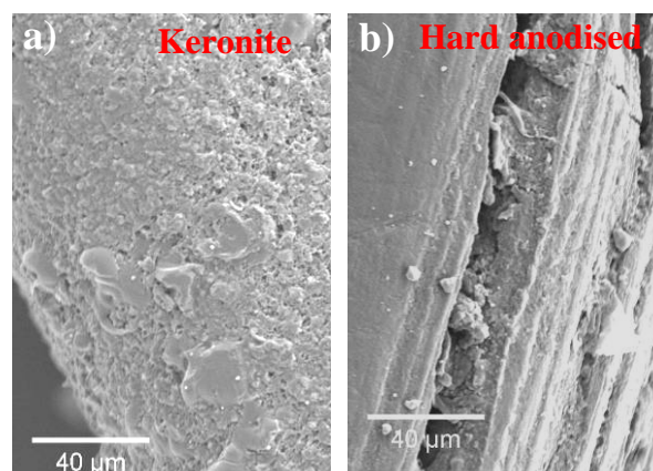
Fig.3 SEM images showing a sharp edge/corner of the coating on AA7075: a) good and uniform coating retention with the Keronite layer; and b) wide-opening cracks with the hard anodised layer[3].
