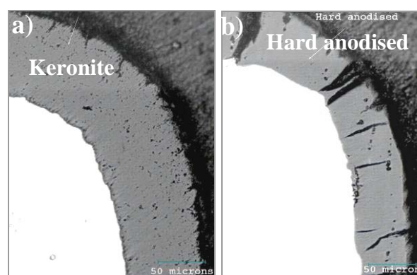
Fig.4 Optical micrographs of: a) Keronite coating showing a uniform coating coverage and good edge retention; and b) hard anodised coating showing extensive V-shaped through thickness columnar cracks extending down to the substrate on the edge.
