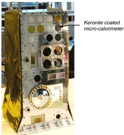
Fig. 14 Keronite coated micro-calorimeter part mounted on the MEDET system for the International Space Station. Courtesy: MEDET Project.
