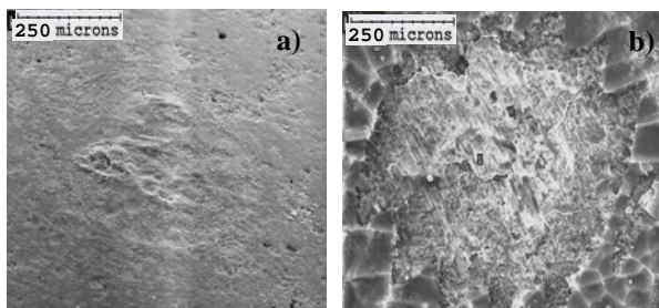
Fig.6. Surface after fretting test of: a) Keronite coating (no visible damage) and b) anodised coating (showing extensive surface cracks) [2]
