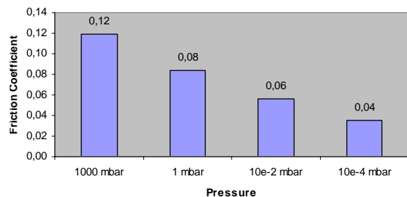
Fig. 7 Friction coefficient of Keronite + MoS 2 composite coating after extreme wear tests in a cryogenic environment. Courtesy: Instituto de Astrofísica de Canarias
