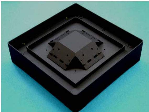
Fig. 13 Coarse sun sensor (CSS) Housing treated with black Keronite.
