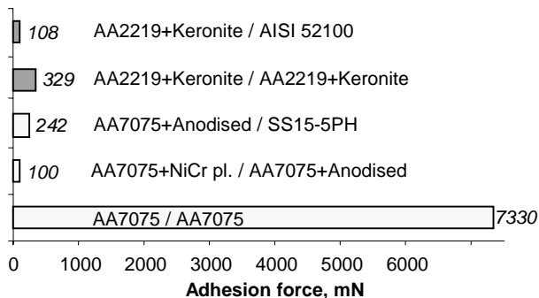
Fig.5. Adhesion measured during fretting tests [2].
