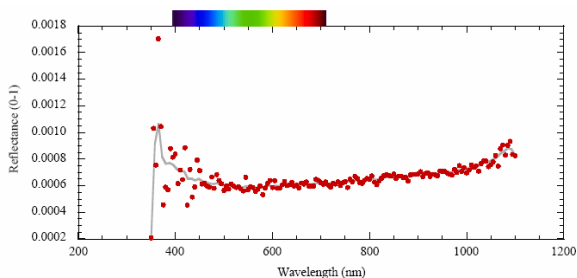
Fig. 9 Reflectance from the surface of a Keronite black sample, measured at 25°C with a fixed angle of incidence of 30 degrees [5].
