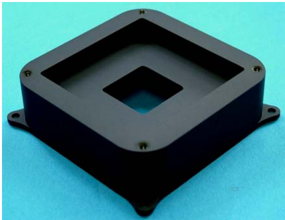
Fig. 12 Fine sun sensor (FSS) Baffle treated with black Keronite.
