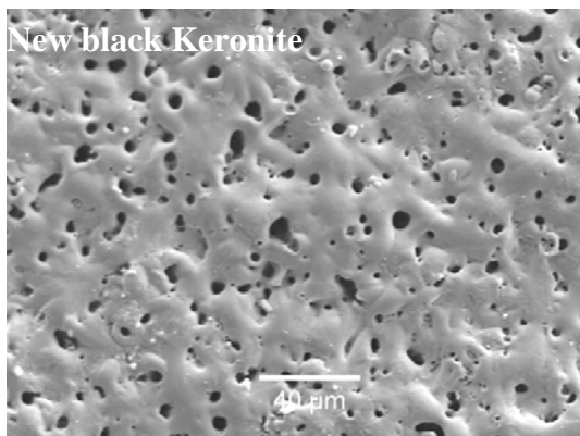
Fig. 8 SEM image of new black Keronite on AA6060 alloy showing coating surface morphology with crater-like porosity.
