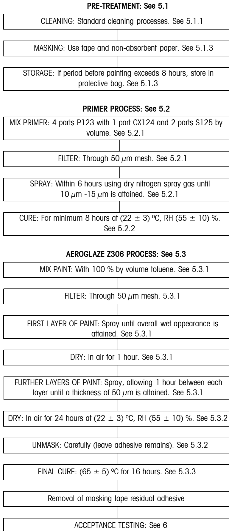
Figure 1: Procedure flow diagram
