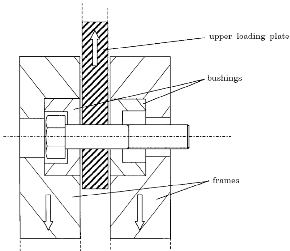
Figure 4-7: Schematic of an example of double-shear loading jigs
