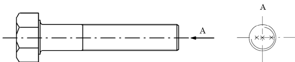
Figure 4-5: Locations for hardness testing (indicated with cross symbol)
