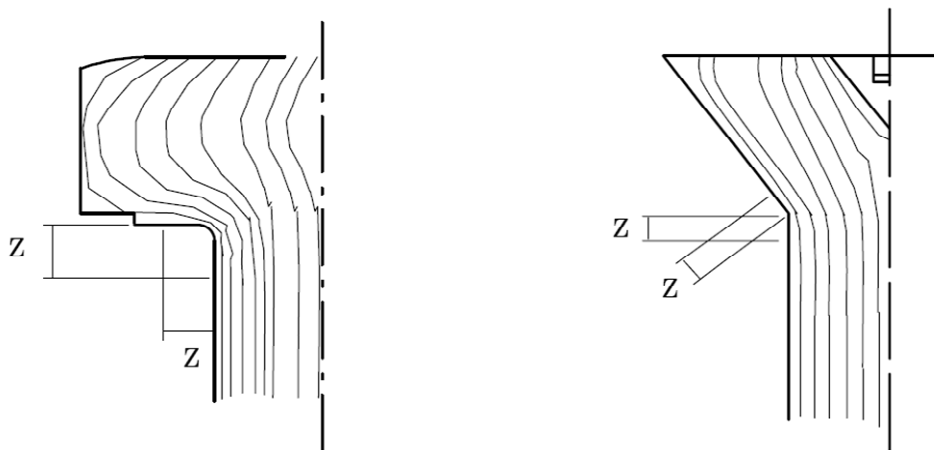
Figure 4-3: Area Z delimiting interruptions in grain flow in the head-to-shank region
